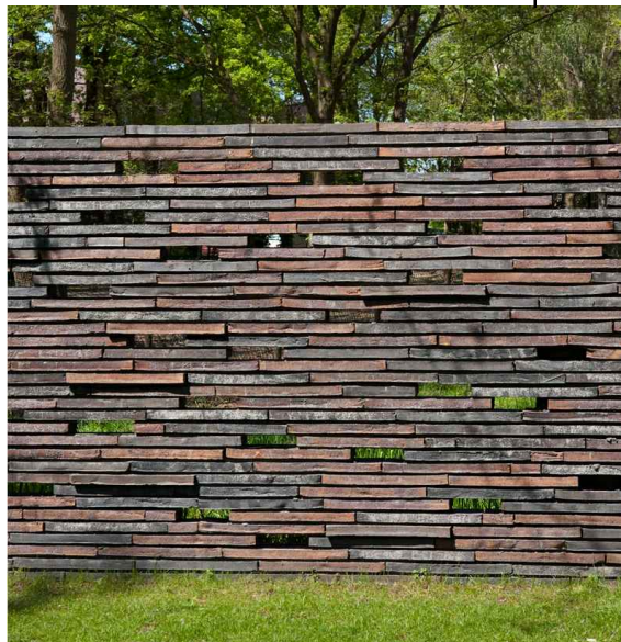
HIT & MISS BOND BRICKWORK. CARPARK ENVELOPE - NATURALLY VENTILATED WALL AS PART OF AN ARCHITECTURAL SCREEN.
