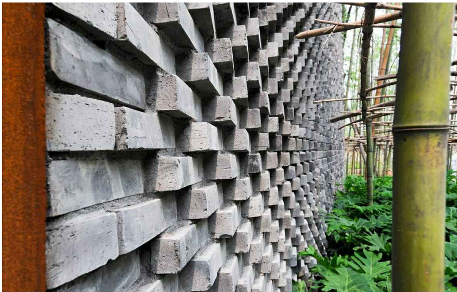
BRICKWORK (TEXTURED BOND) / INTEGRATED PLANTER BOX.
